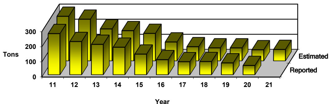
Figure 13 Sulfur Dioxide Emission Trend (1000s of Tons/Year)
