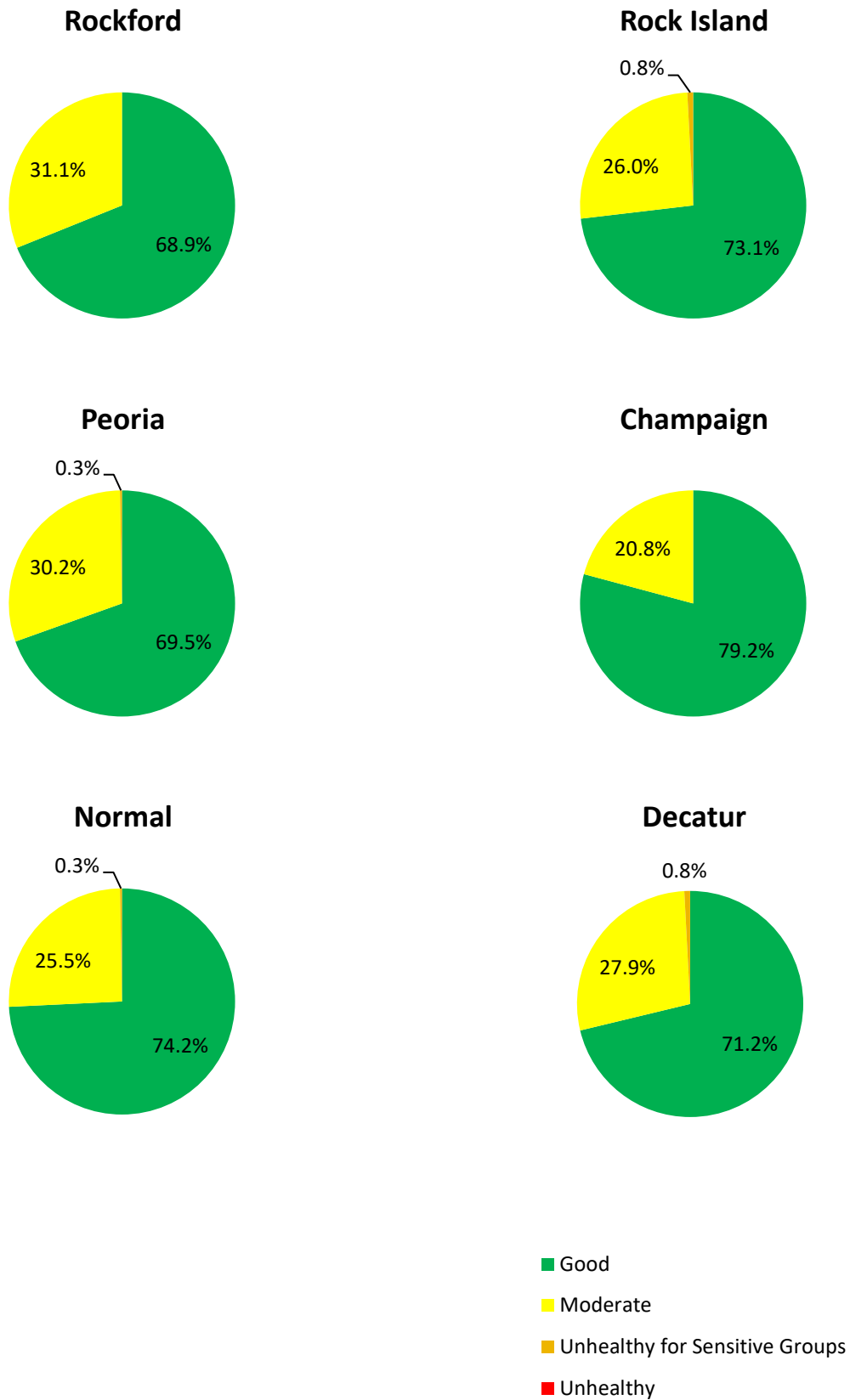
Figure 9: 2021 Air Quality Index Summaries by Sector
